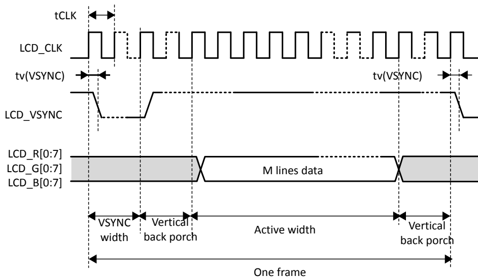
Figure 56. LCD-TFT vertical timing diagram
