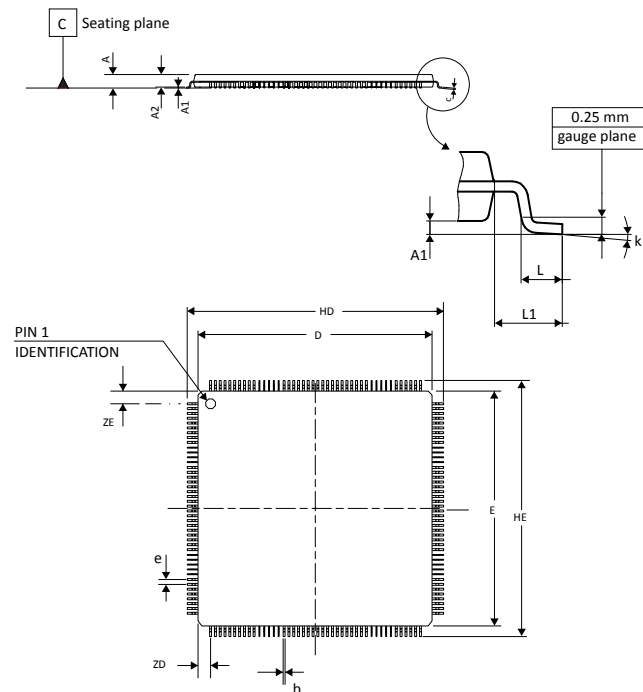
Figure 82. LQFP - 176 pins, 24 x 24 mm low profile quad flat package outline
