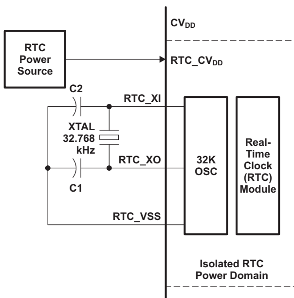
Figure 6-85. Clock Source
