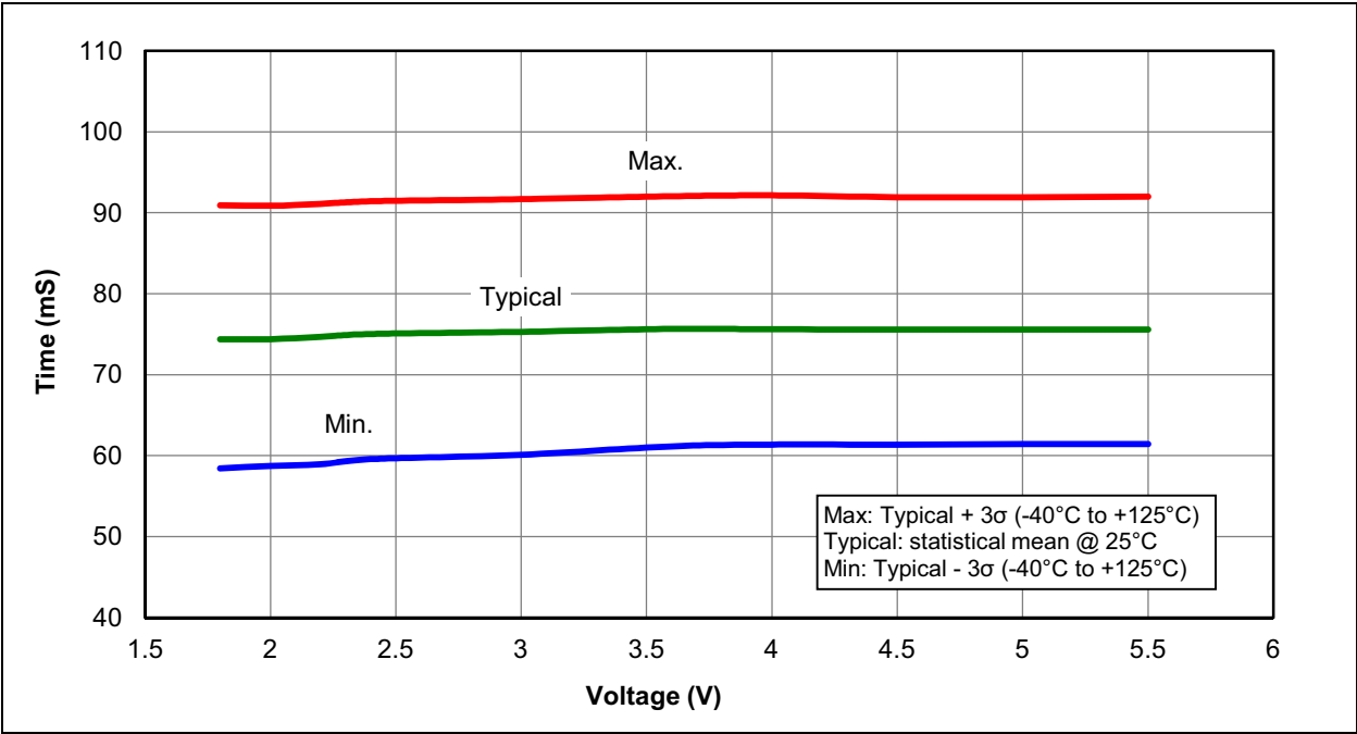
FIGURE 31-62: PWRT PERIOD
