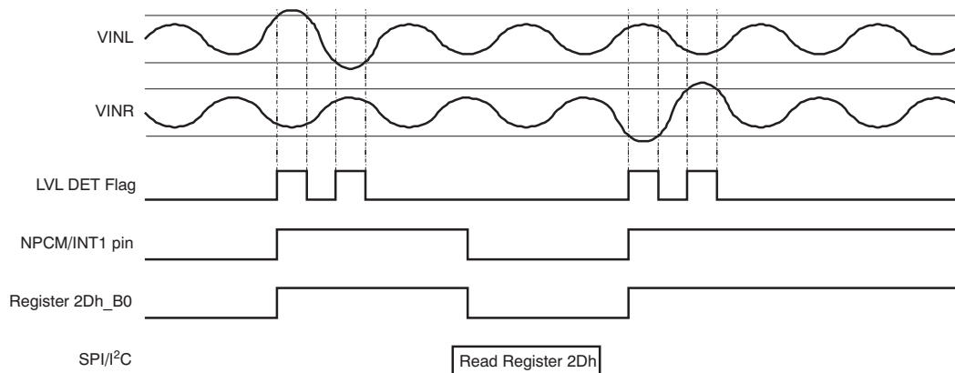
Figure 20. Operation of the ADC Level Detect Circuitry
