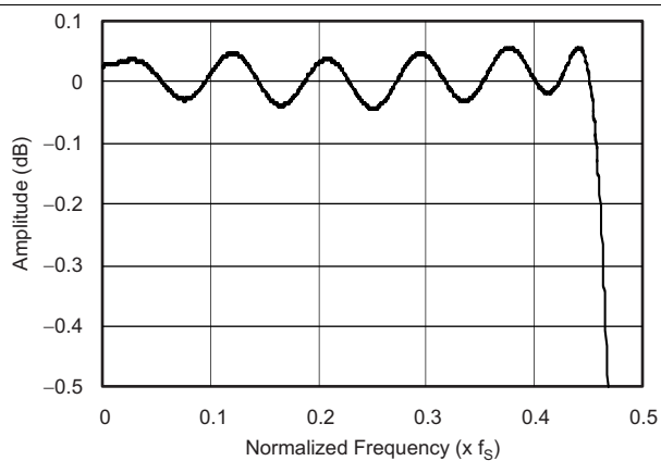
Figure 6. Decimation Filter Passband Characteristic
