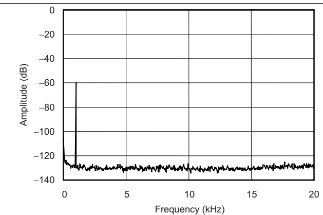
Figure 10. Output Spectrum
