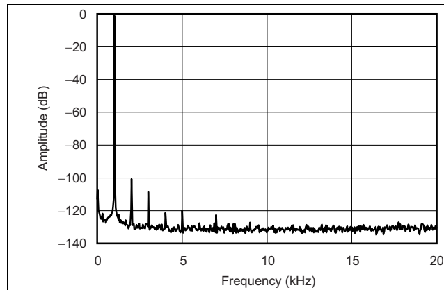
Figure 9. Output Spectrum
