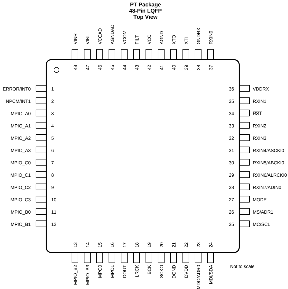
Pin Functions
