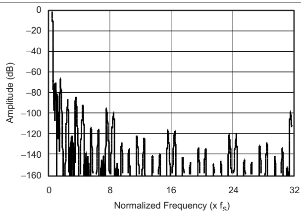
Figure 5. Decimation Filter Stop Band Characteristic
