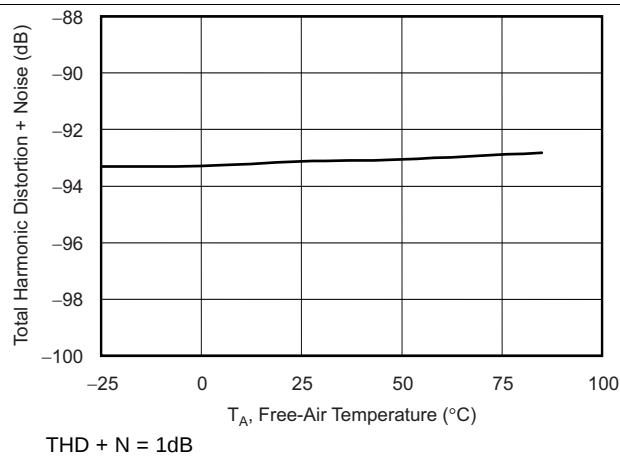
Figure 1. Total Harmonic Distortion + Noise vs Temperature
