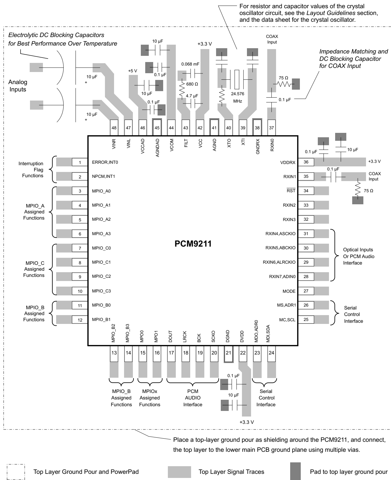
Figure 109. Layout Example
