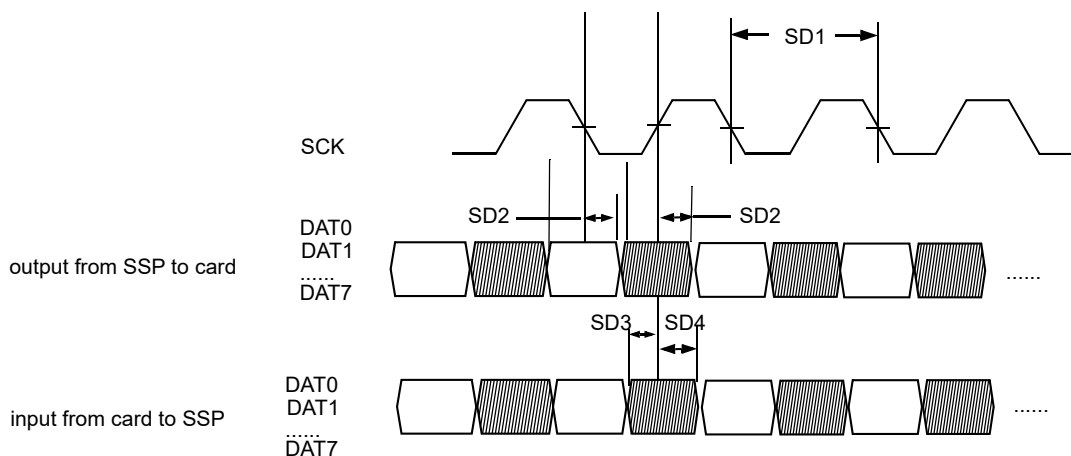
Figure 37. MMC4.4 Timing
