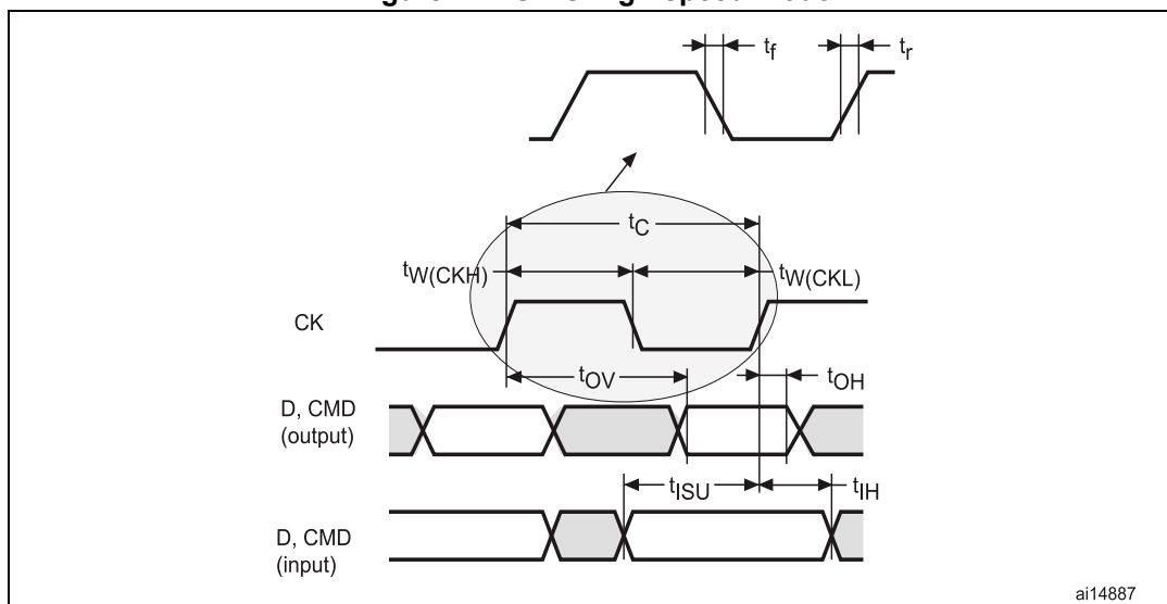
Figure 111. SDIO high-speed mode
