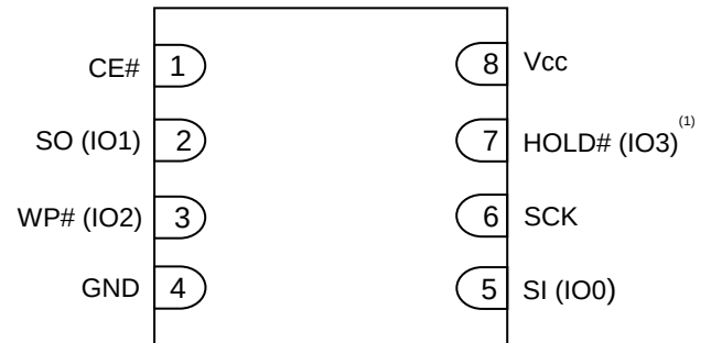
8-contact WSON 6x5mm 8-contact WSON 8x6mm 8-contact USON 4x3mm
