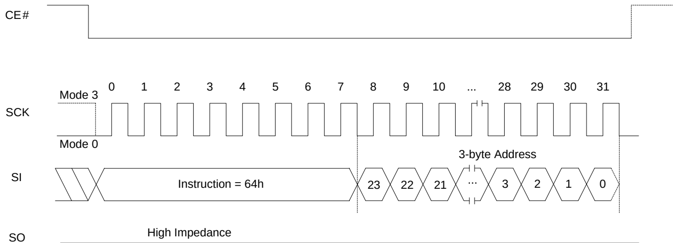
Figure 8.48 IRER COMMAND (Information Row Erase) OPERATION
