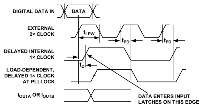
Figure 34. Internal Timing of AD9772A with PLL Disabled
