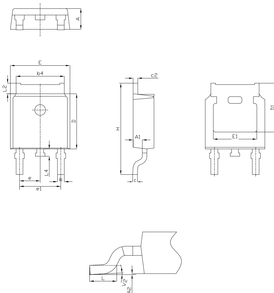
Figure 15. DPAK (TO-252) package outline H
