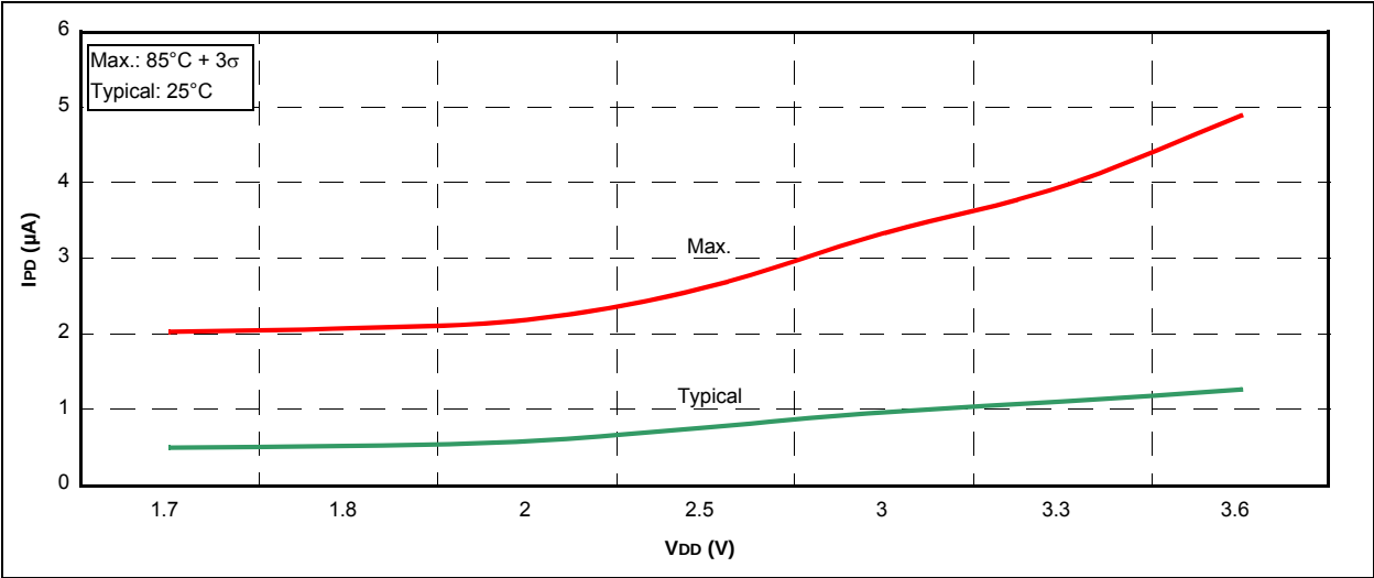
FIGURE 31-41: PIC16LF1937 LCD, LOW POWER
