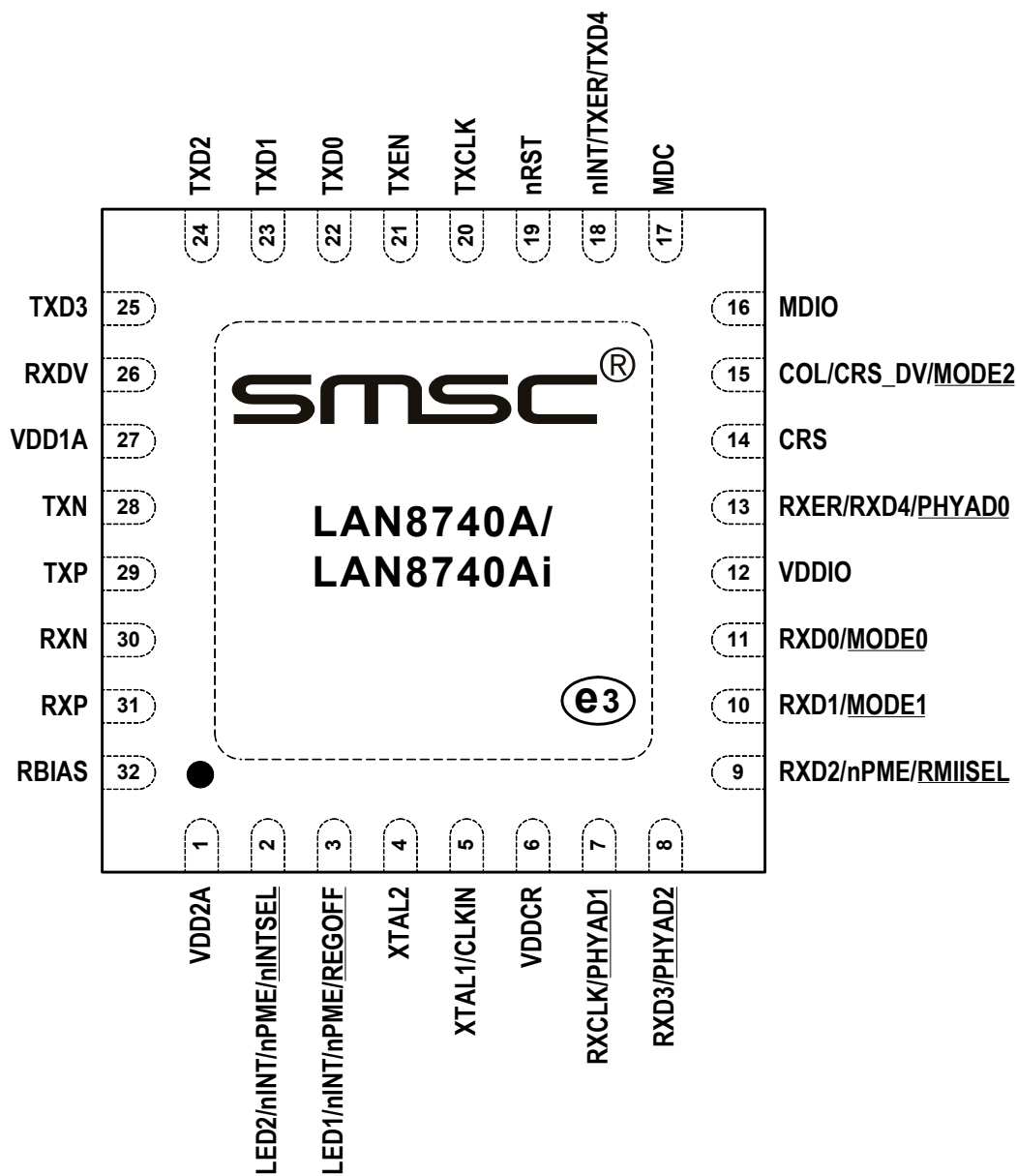
Figure 2.1 32-SQFN Pin Assignments (TOP VIEW)
