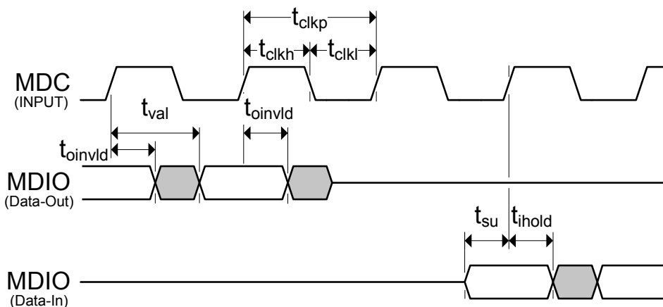
Figure 5.7 SMI Timing
