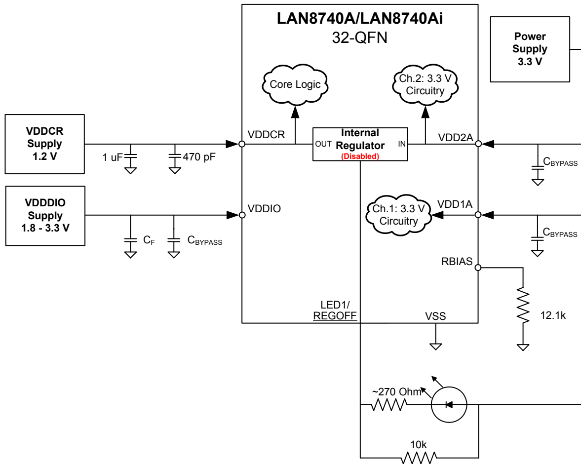
Figure 3.19 Power Supply Diagram (1.2 V Supplied by External Source)
