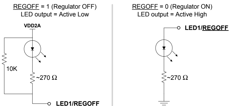
Figure 3.11 LED1/REGOFF Polarity Configuration
