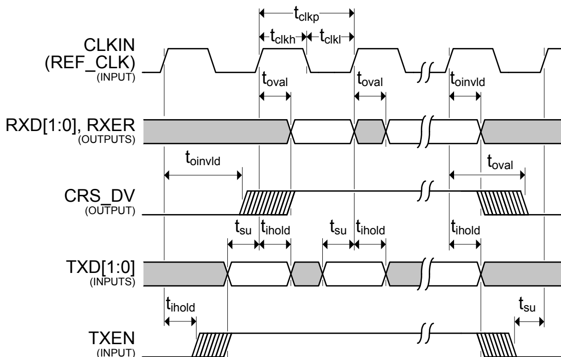
Figure 5.6 RMII Timing
