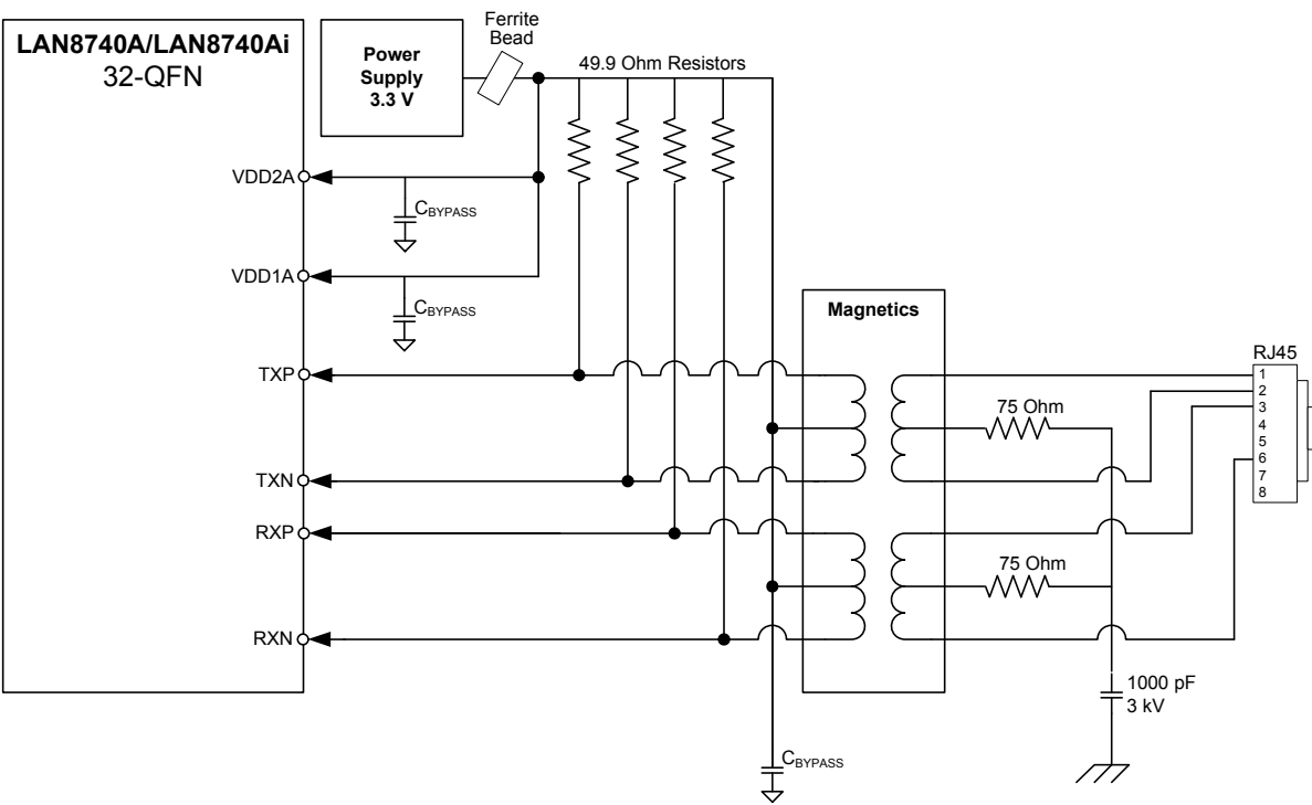
Figure 3.20 Twisted-Pair Interface Diagram (Single Power Supply)
