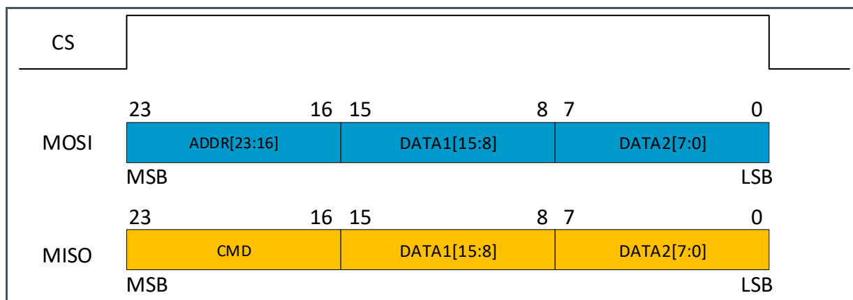
Figure 15: Read/Write Command
