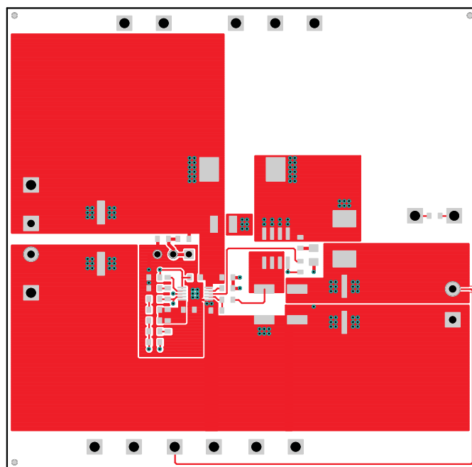
Figure 38. Top Copper
